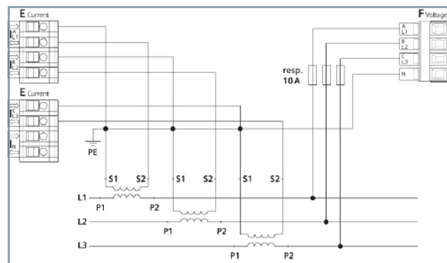
Figure 2.3/8 Connection Example 3-Wire Network, 3 Current Transformers, Any Load
