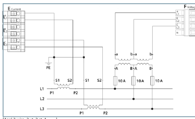
Figure 3.1/11 Connection Example 3-Wire Network, 2 Voltage and 2 Current Transformers. Any Load
