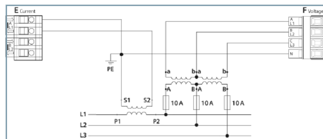
Figure 2.3/9 Connection Example 3-Wire Network, 2 Voltage Transformers and 1 Current Transformer, Same Load
