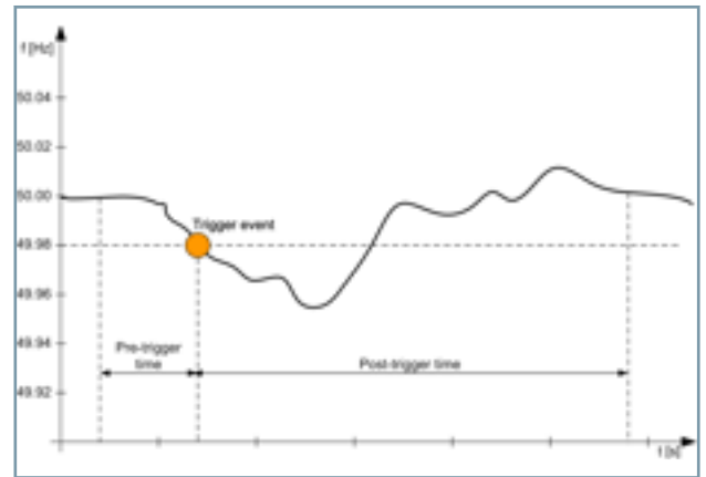
Figure 6.3/7 Automatic Time Trigger (for the Frequency, for Example)
