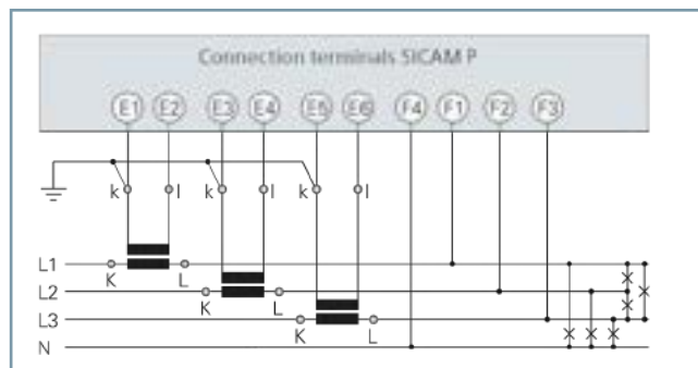
Figure 3.3/18 4 Conductors, 3 Phases (Low-Voltage System) 1,2
