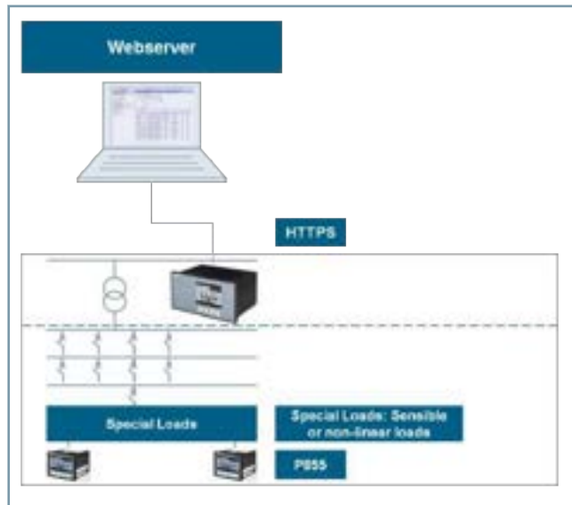
Figure 2.2/3 Standalone Analyzer
