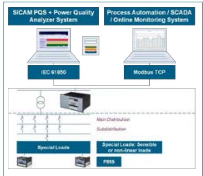
Figure 2.2/5 Application Example in the Industry
