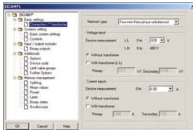
Figure 3.3/10 Parameterization
