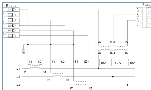
Figure 3.1/12 Connection Example 3-Wire Network, 2 Voltage and 3 Current Transformers, Any Load
